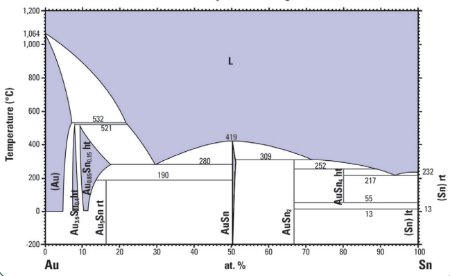
AuSn Binary Phase Diagram
