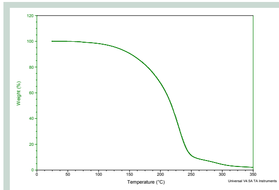
TGA was performed at a ramp rate of 10 °C per minute.
